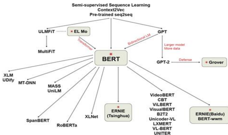
Figure 3. The academic evolution of word embedding methods.
